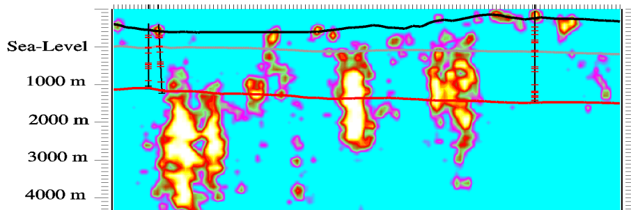
Figure 2: (a) North-South and (b) East-West section through a Werner depth volume for an area east of the PRA. Wells shown in (b) with formation picks, Precambrian in red, Debolt in grey and surface in black. Wells projected to the line. Sections are about 50 km long.
