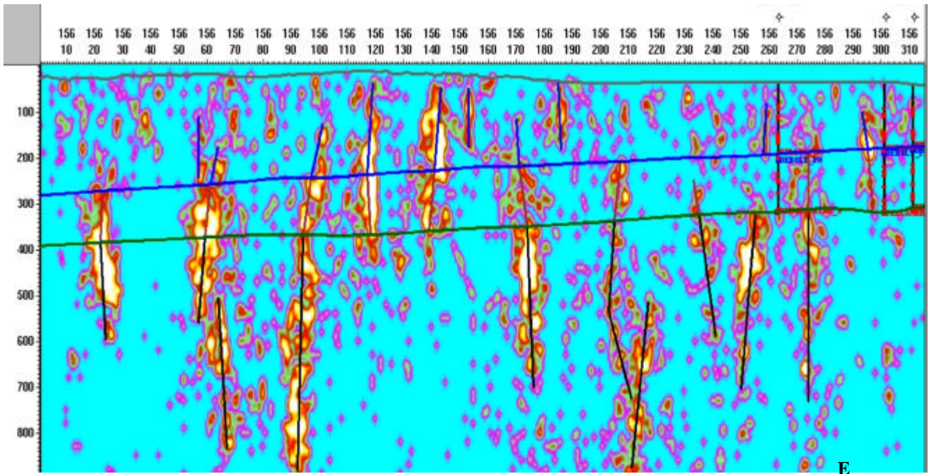
Figure 1: An east west MaFIC section through a Werner depth solution volume for an area over the PRA. Wells at east of line were used to pick formation depths. Blue is Debolt and Green is Precambrian. Near vertical fault traces, in black, are interpreted on the depth solutions. Line is about 120 km long.
